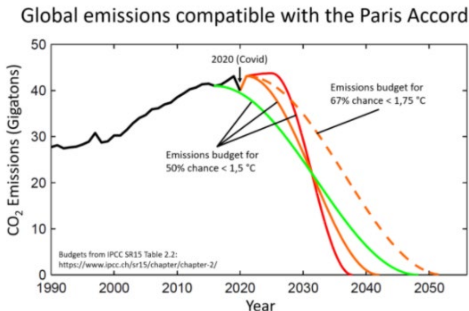
Figure 3, Emission trajectories required to meet Paris Accord targets. Source: RealClimate: ‘Two graphs show the path to 1.5 degrees’
