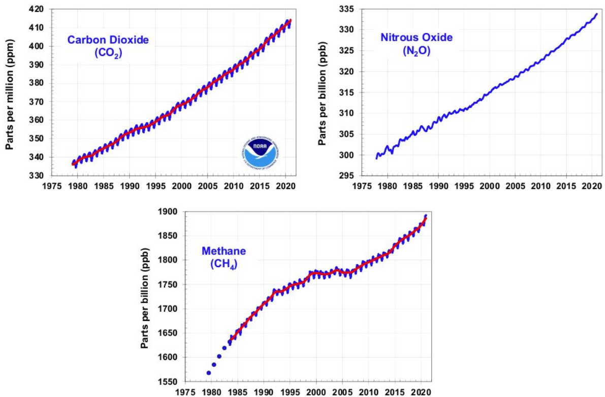
Figure 2, Graphs showing concentrations of CO 2 , N 2 O and CH 4 Source: https://www.co2.earth/annual-ghg-index-aggi
